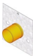
End cap with horizontal PVC-U pipe outlet DN/OD 160, type 020
